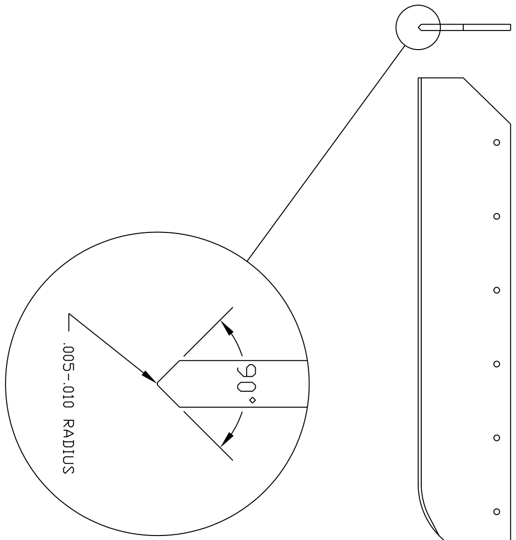
EDGE DETAIL VIEWED FROM BACK
